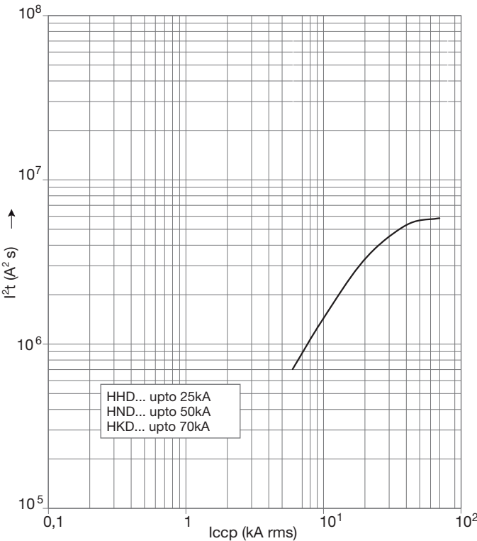
MCCB h400 TM (400A)
