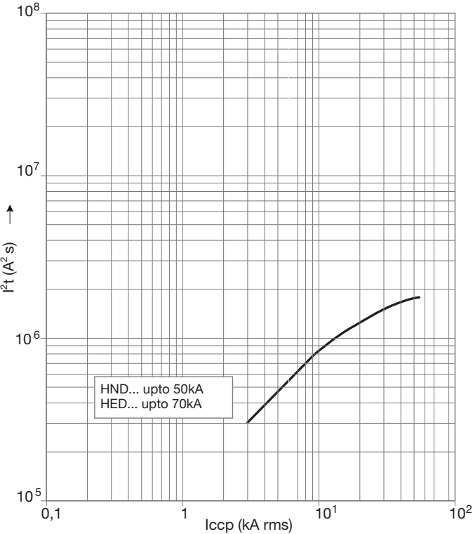
MCCB h630 LSI (250A)
