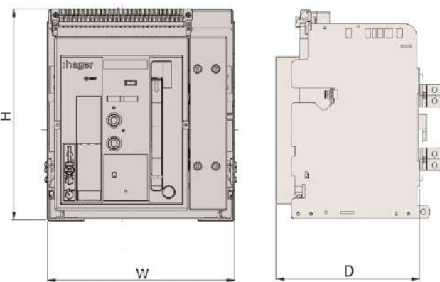
Draw-out type
