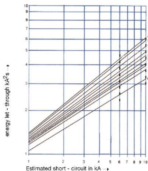
i^2t characteristics curve
