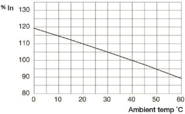
Temperature compensation curve (front connection)
