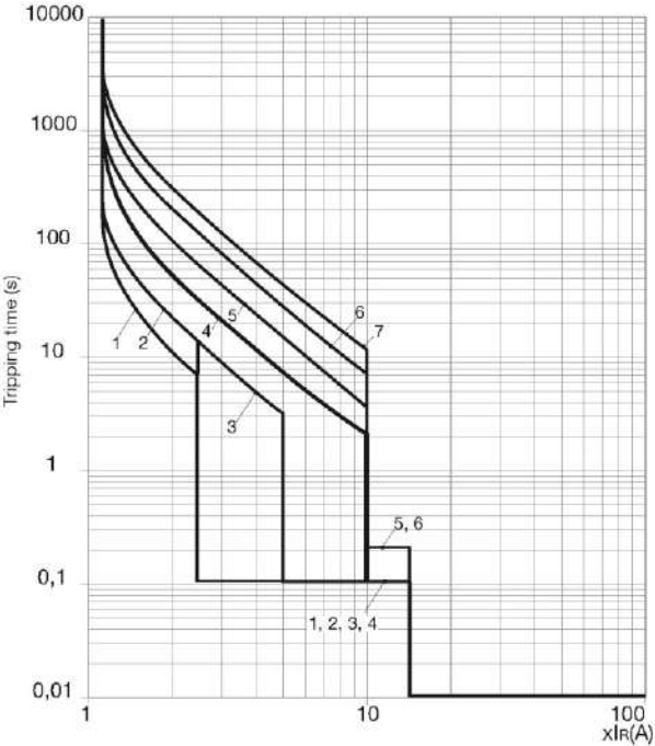
MCCB h630 LSI (250A and 400A)
