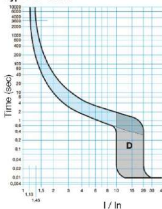
Type "D" curve
