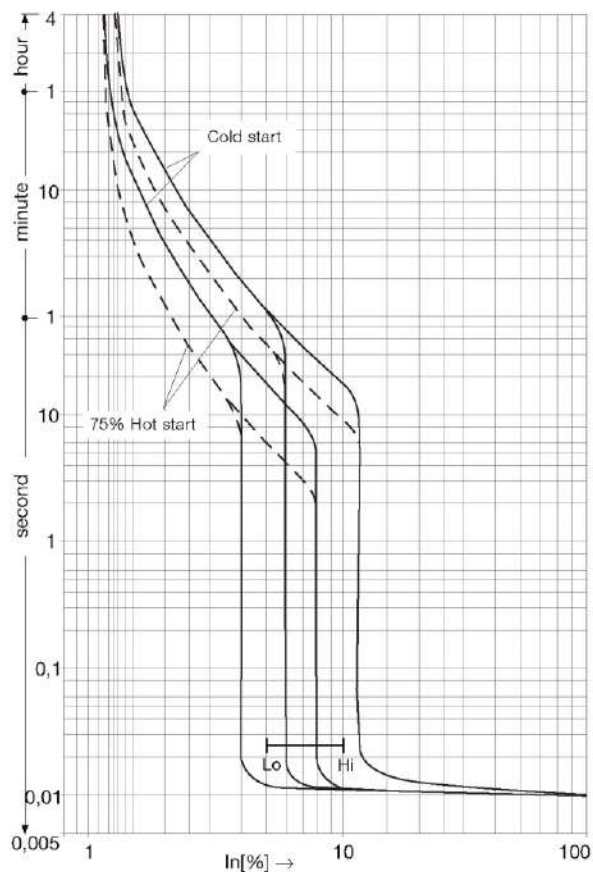
MCCB h800 TM (800A)
