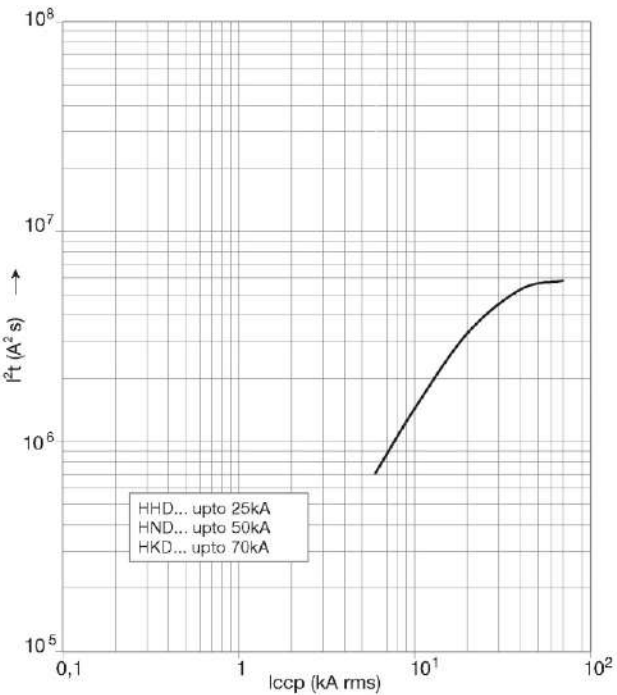
MCCB h400 TM (400A)
