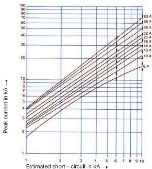
Current limitation curve
