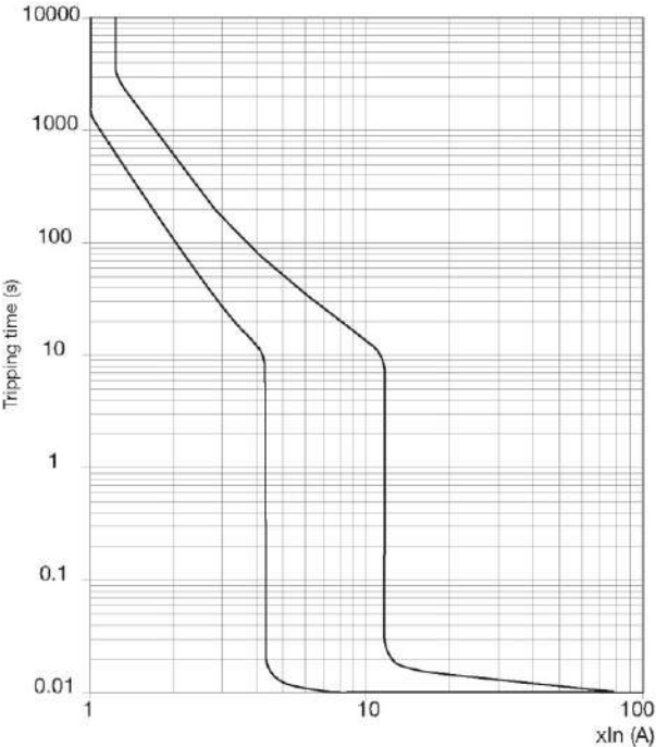
MCCB h400 TM (250 and 400A)
