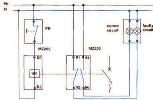
Emergency switch - off with under voltage release
