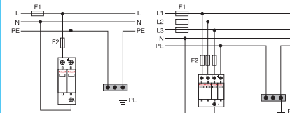
TT System HDY3N Installation Diagram
