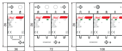
Overall Dimension of HDY3N-80 and 120
