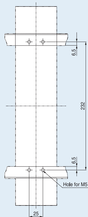
Mounting dimensions
