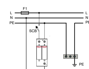
TT System Installation Diagram
