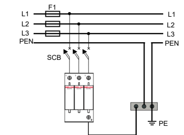
TN-C System Installation Diagram
