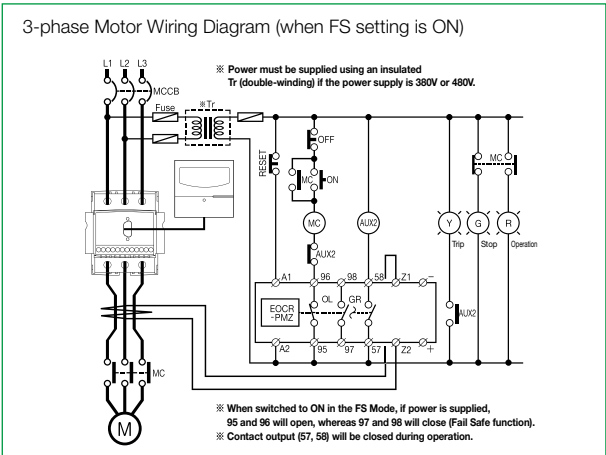
EOCR-PFZ (Terminal Type)
