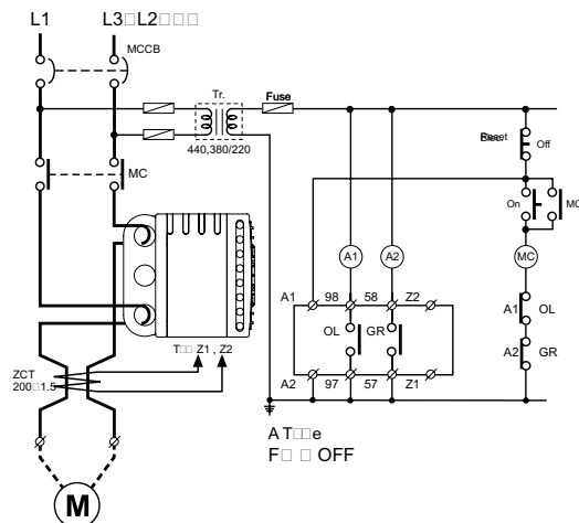
Single phase motor (A type)
