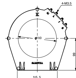
ZCT-Ø120
